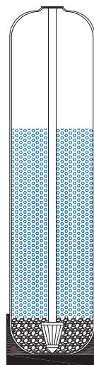
Standard Tank
